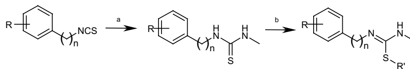
Scheme 1. Reagents and conditions: (a) 4 equiv methylamine, acetone, rt, 8 h; (b) 1.1 equiv R'I, K 2 CO 3 , DMF, rt, 12 h.
